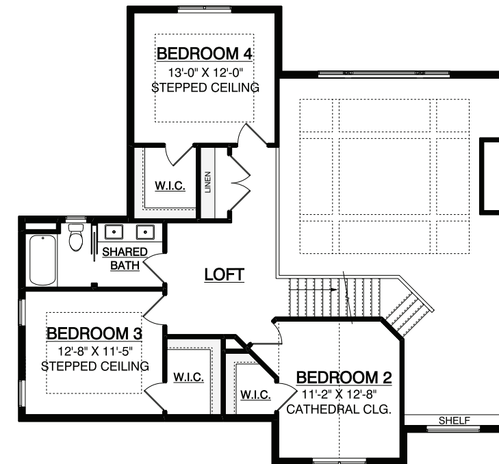
SECOND FLOOR 871 SQ. FT.
